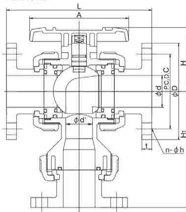
FLANGED
