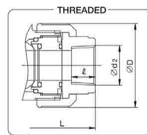
THREADED
