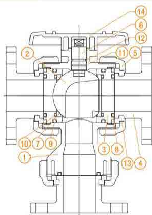
FLANGED
