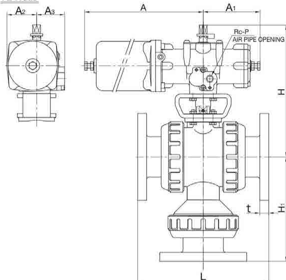
FLANGED
