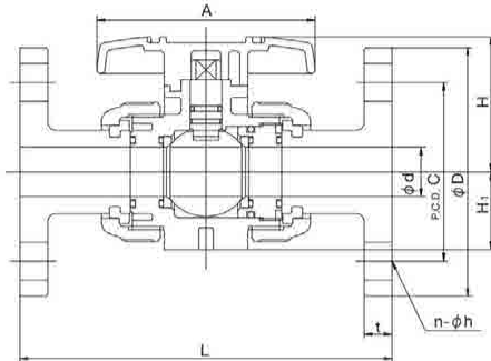
FLANGED
