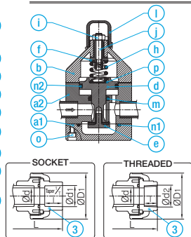
15 mm — 40 mm V182 INSIDE STRUCTURE DIAGRAM
