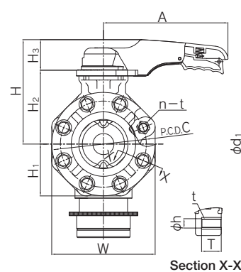
Section X-X
