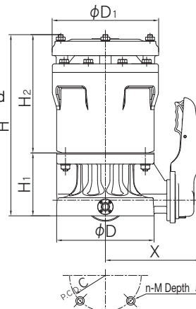
100 mm – 200 mm (4 inch – 8 inch) FLANGED
