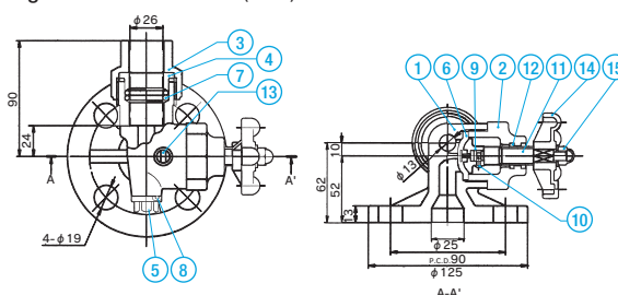
Gauge valve JIS 10K: 25 mm (1 inch)
