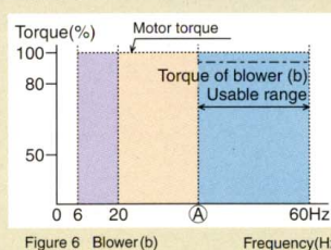
Figure 6 Blower(b) Frequency(Hz)
