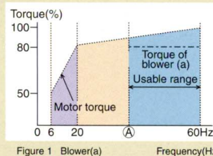
Figure 1 Blower(a) Frequency(Hz)
