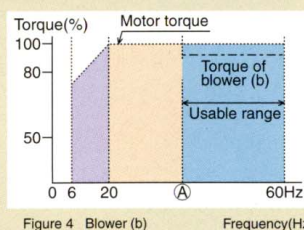
Figure 4 Blower(b) Frequency(Hz)
