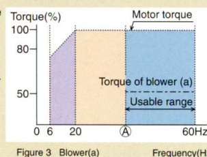
Figure 3 Blower(a) Frequency(Hz)
