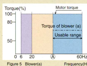
Figure 5 Blower(a) Frequency(Hz)
